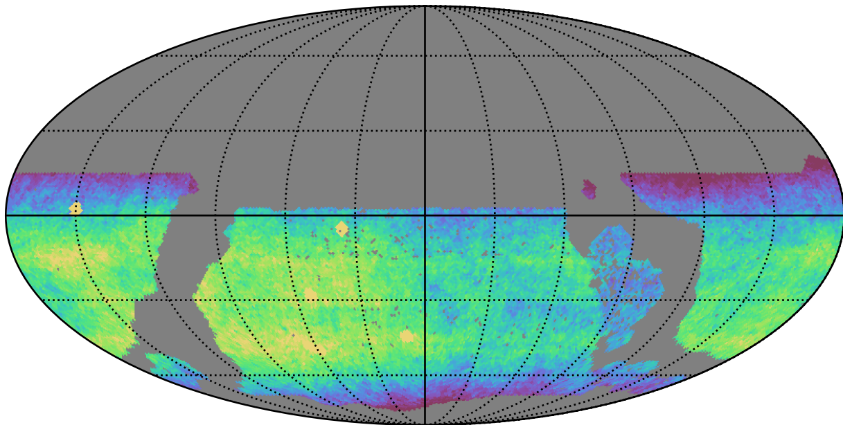
early_u_fpextra2.0_v3.4_10yrs WFD z band: CoaddM5
