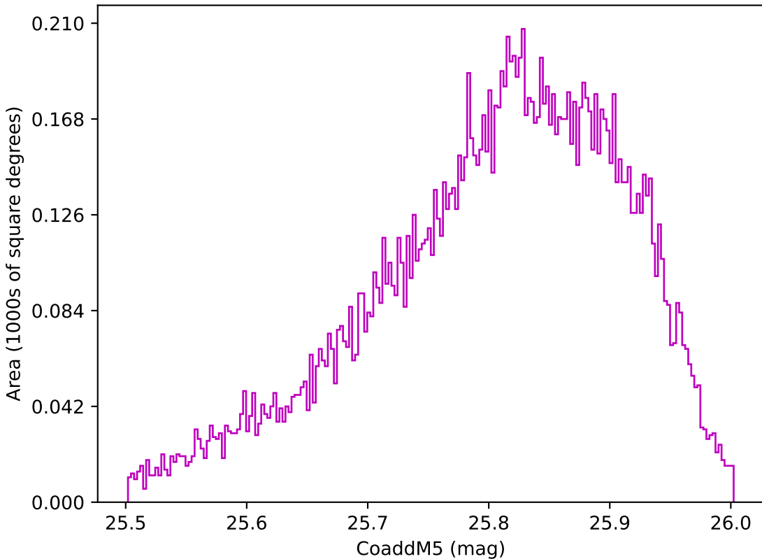
early_u_fpextra2.0_v3.4_10yrs WFD z band: CoaddM5
