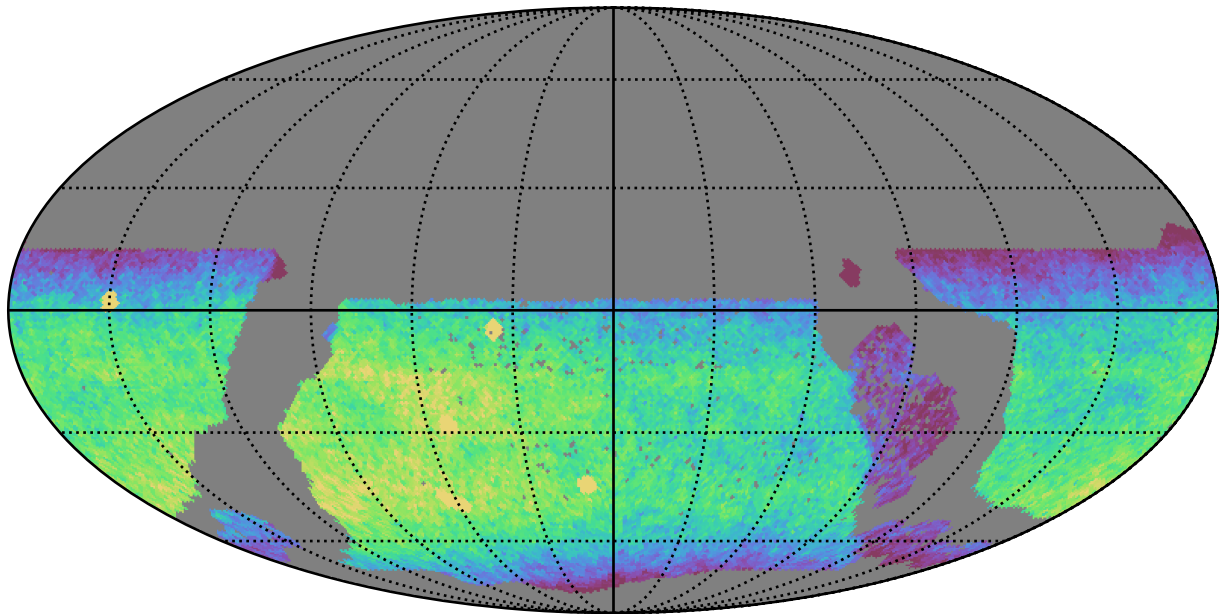
early_u_fpextra2.0_v3.4_10yrs WFD y band: CoaddM5
