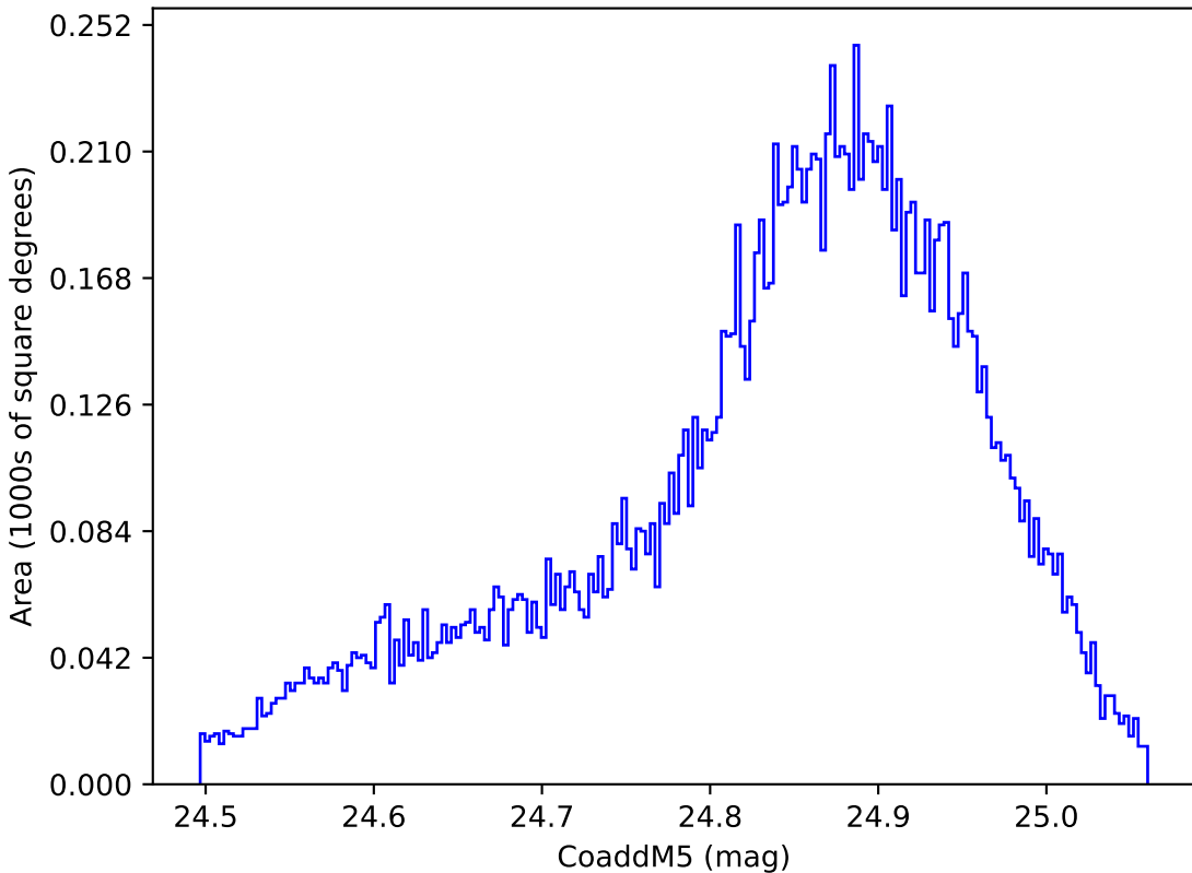
early_u_fpextra2.0_v3.4_10yrs WFD y band: CoaddM5
