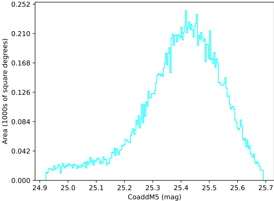
early_u_fpextra2.0_v3.4_10yrs WFD u band: CoaddM5
