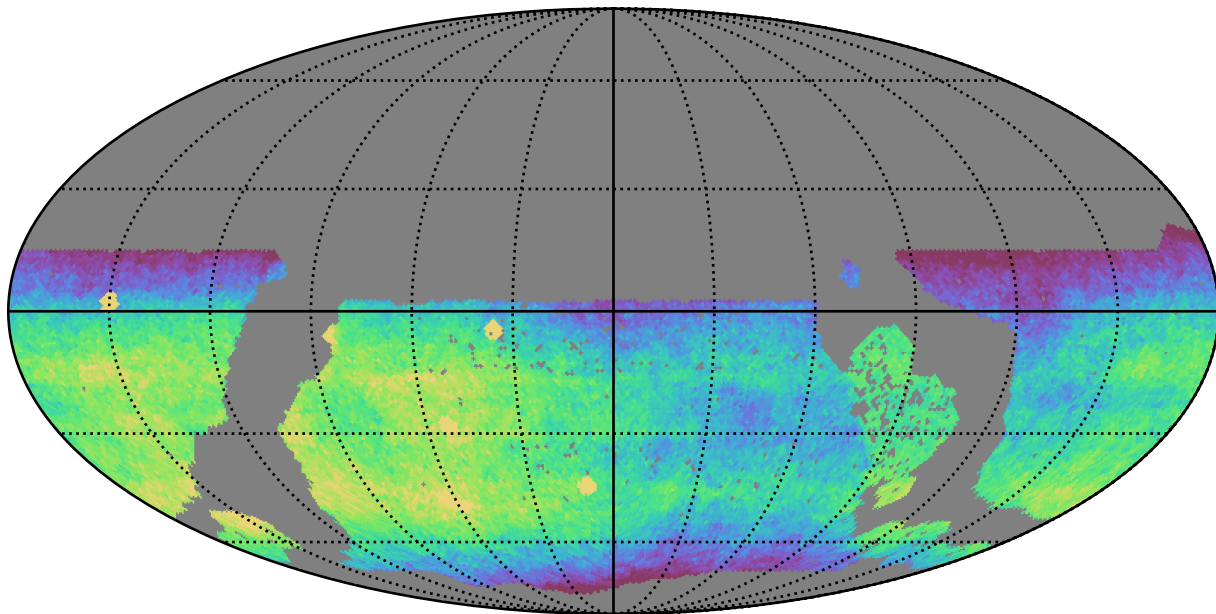
early_u_fpextra2.0_v3.4_10yrs WFD r band: CoaddM5
