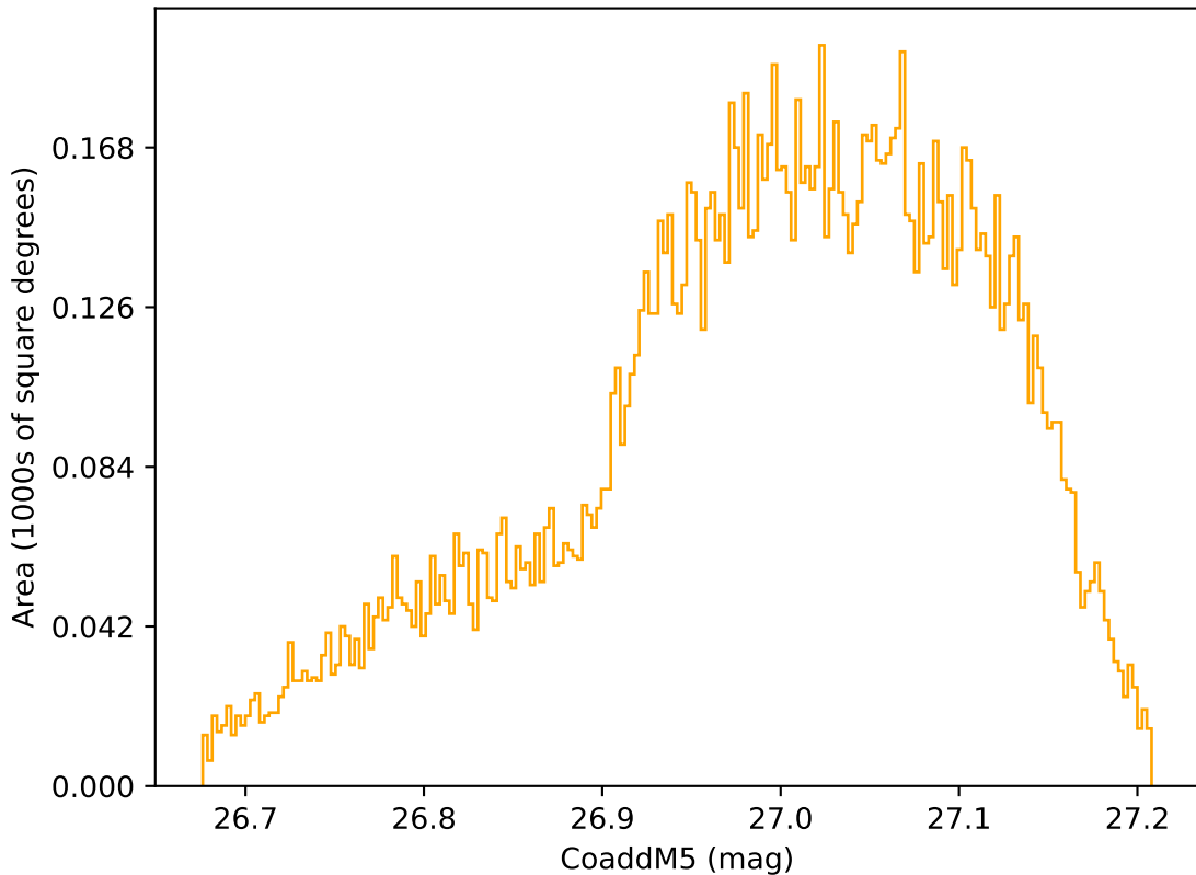
early_u_fpextra2.0_v3.4_10yrs WFD r band: CoaddM5
