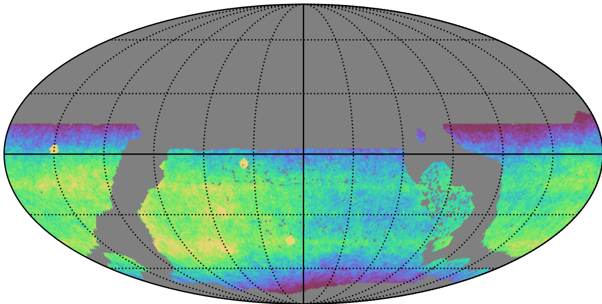
early_u_fpextra2.0_v3.4_10yrs WFD i band: CoaddM5
