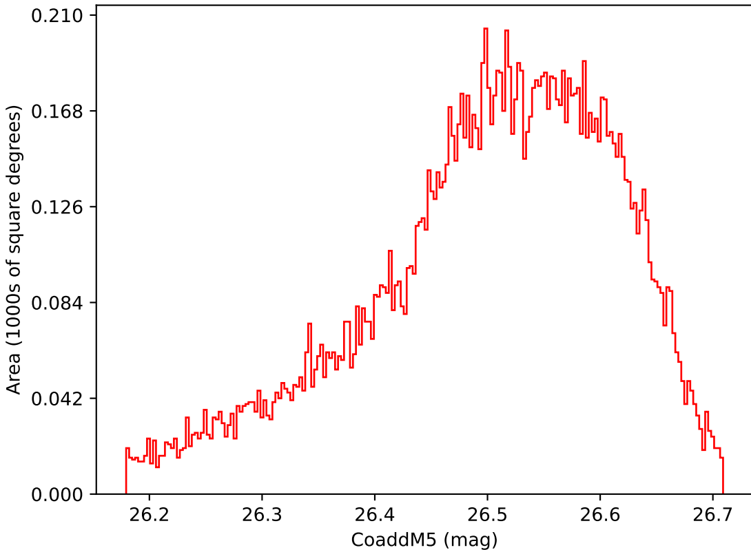
early_u_fpextra2.0_v3.4_10yrs WFD i band: CoaddM5
