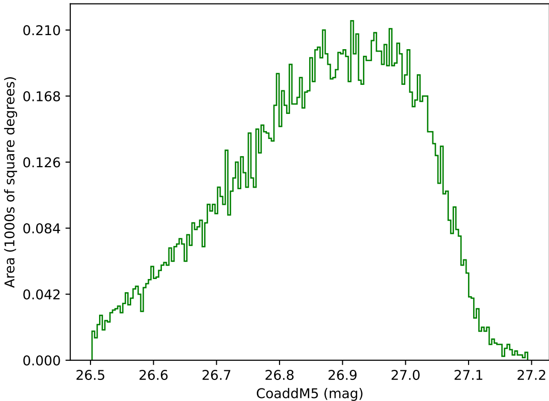
early_u_fpextra2.0_v3.4_10yrs WFD g band: CoaddM5
