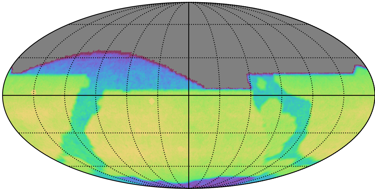
early_u_fpextra2.0_v3.4_10yrs All sky z band: CoaddM5
