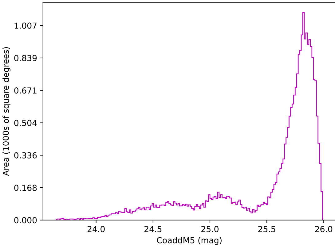
early_u_fpextra2.0_v3.4_10yrs All sky z band: CoaddM5
