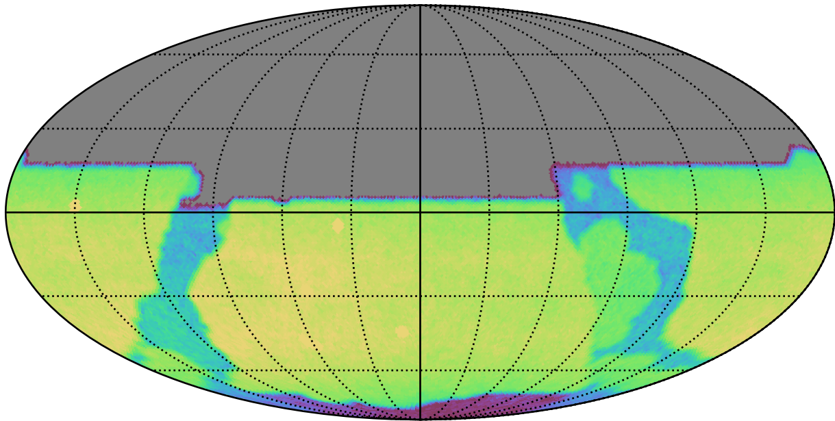
early_u_fpextra2.0_v3.4_10yrs All sky y band: CoaddM5
