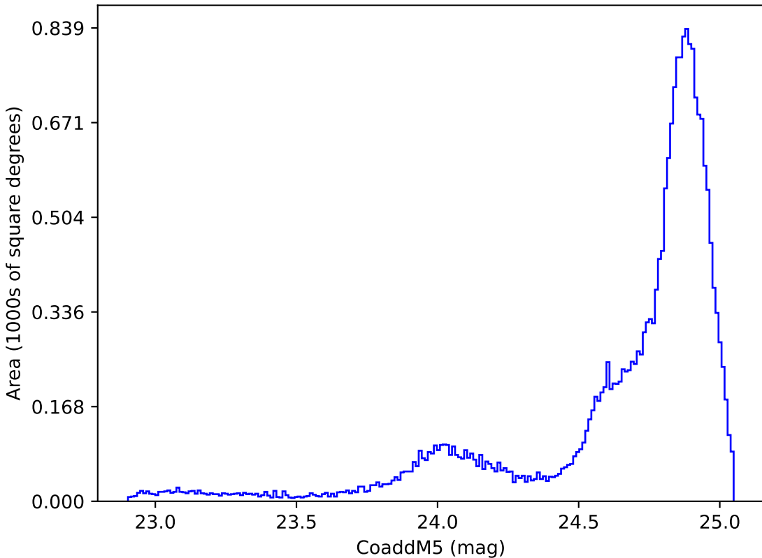
early_u_fpextra2.0_v3.4_10yrs All sky y band: CoaddM5
