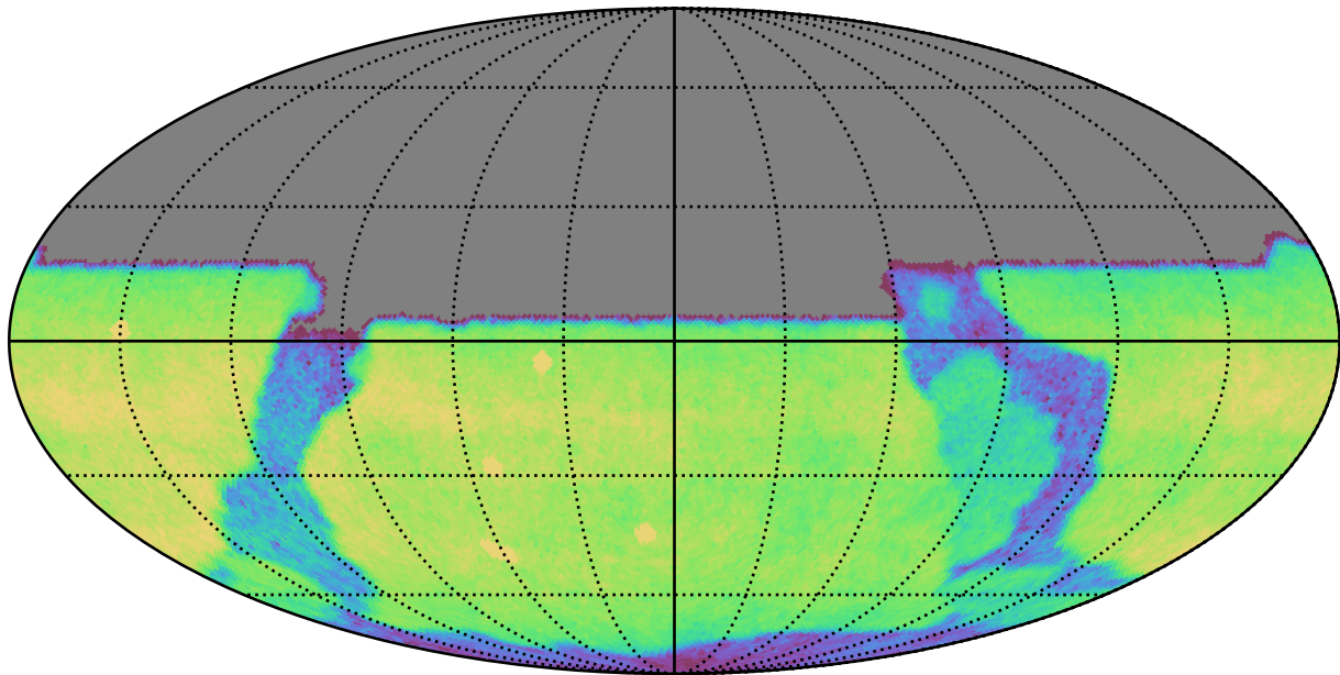
early_u_fpextra2.0_v3.4_10yrs All sky u band: CoaddM5
