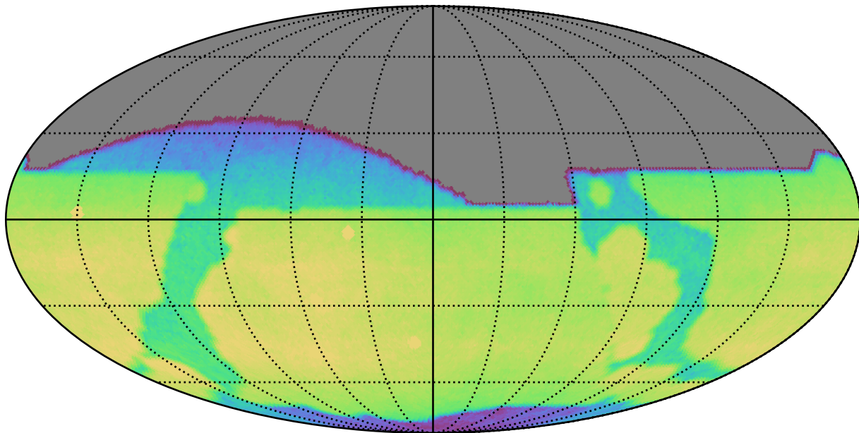
early_u_fpextra2.0_v3.4_10yrs All sky r band: CoaddM5
