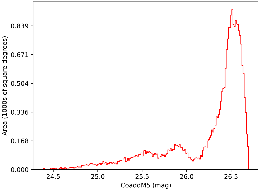
early_u_fpextra2.0_v3.4_10yrs All sky i band: CoaddM5
