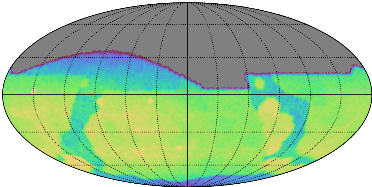
early_u_fpextra2.0_v3.4_10yrs All sky g band: CoaddM5
