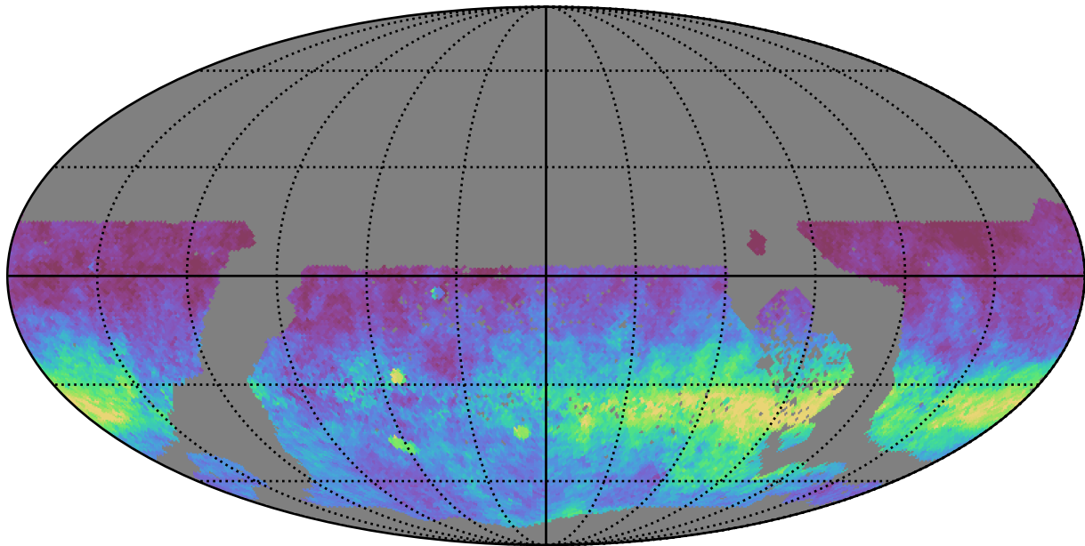
early_u_fpextra2.0_v3.4_10yrs WFD z band: AngleRms rotSkyPos
