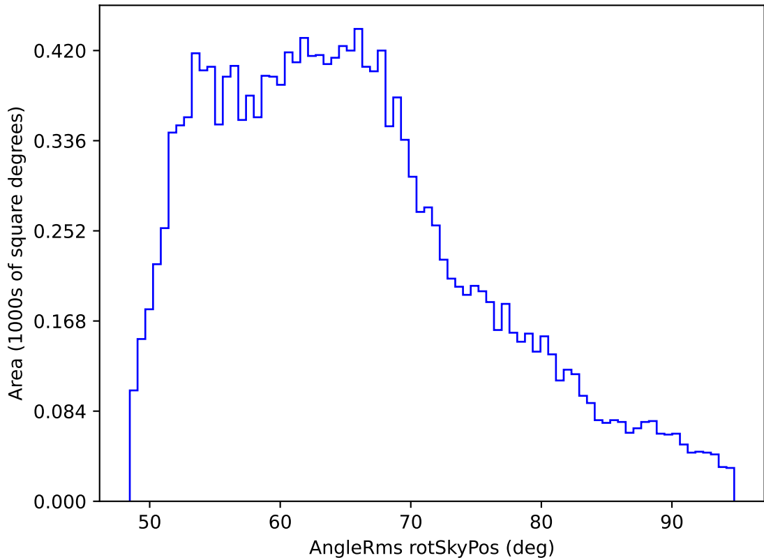
early_u_fpextra2.0_v3.4_10yrs WFD z band: AngleRms rotSkyPos
