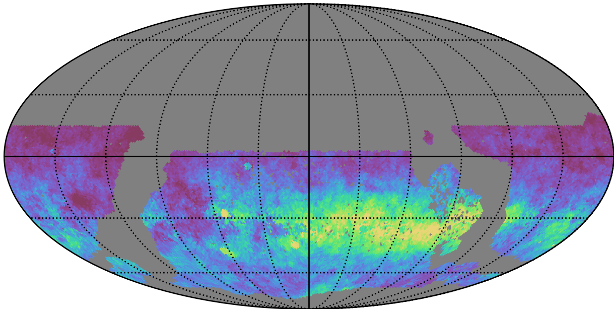
early_u_fpextra2.0_v3.4_10yrs WFD y band: AngleRms rotSkyPos
