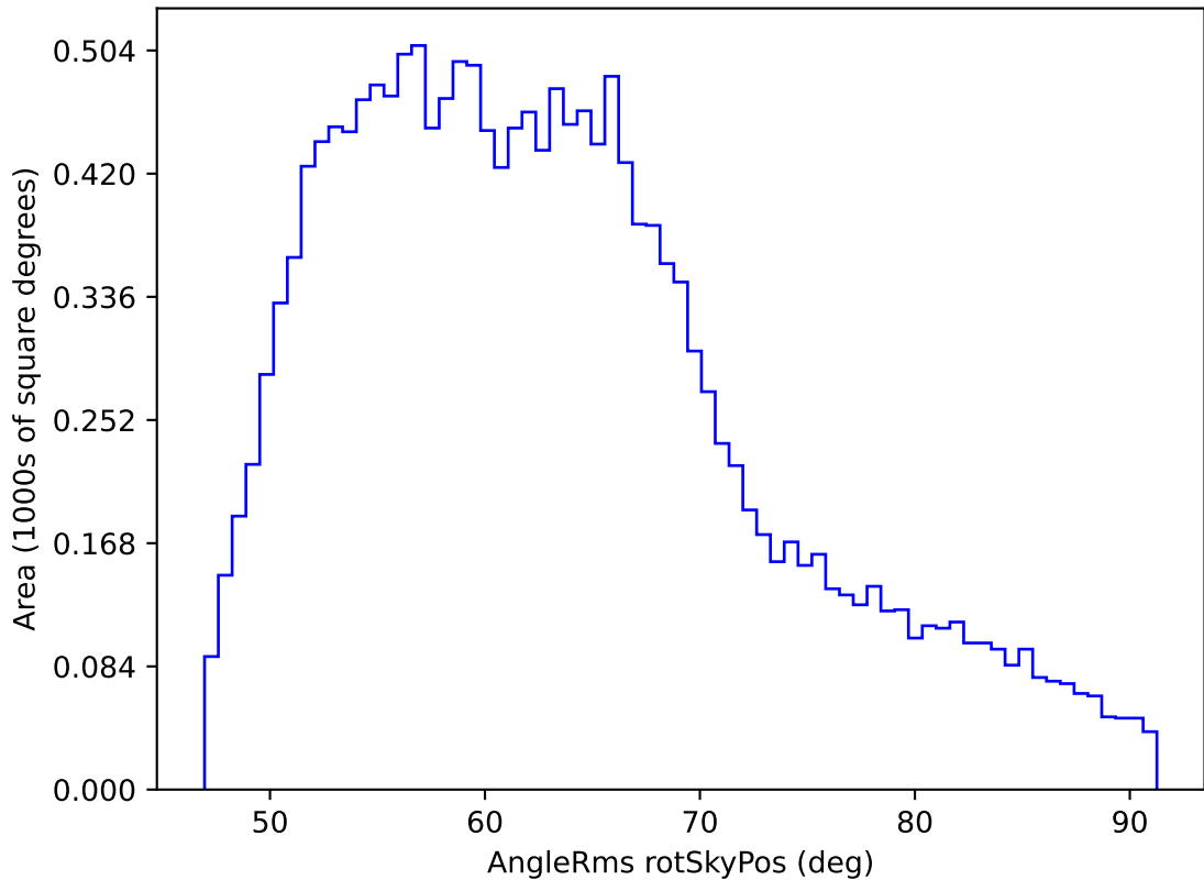
early_u_fpextra2.0_v3.4_10yrs WFD y band: AngleRms rotSkyPos
