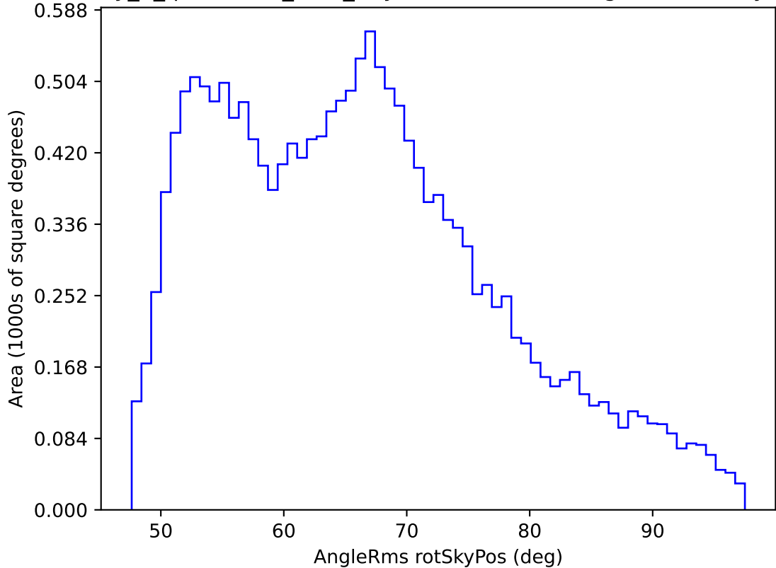
early_u_fpextra2.0_v3.4_10yrs WFD r band: AngleRms rotSkyPos
