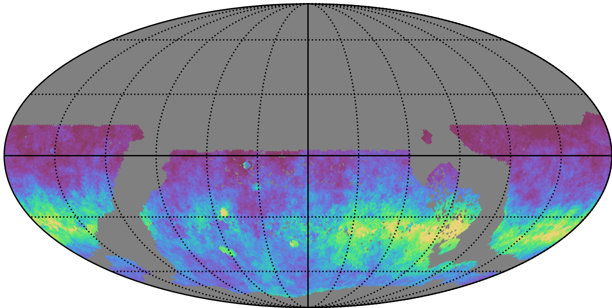
early_u_fpextra2.0_v3.4_10yrs WFD i band: AngleRms rotSkyPos
