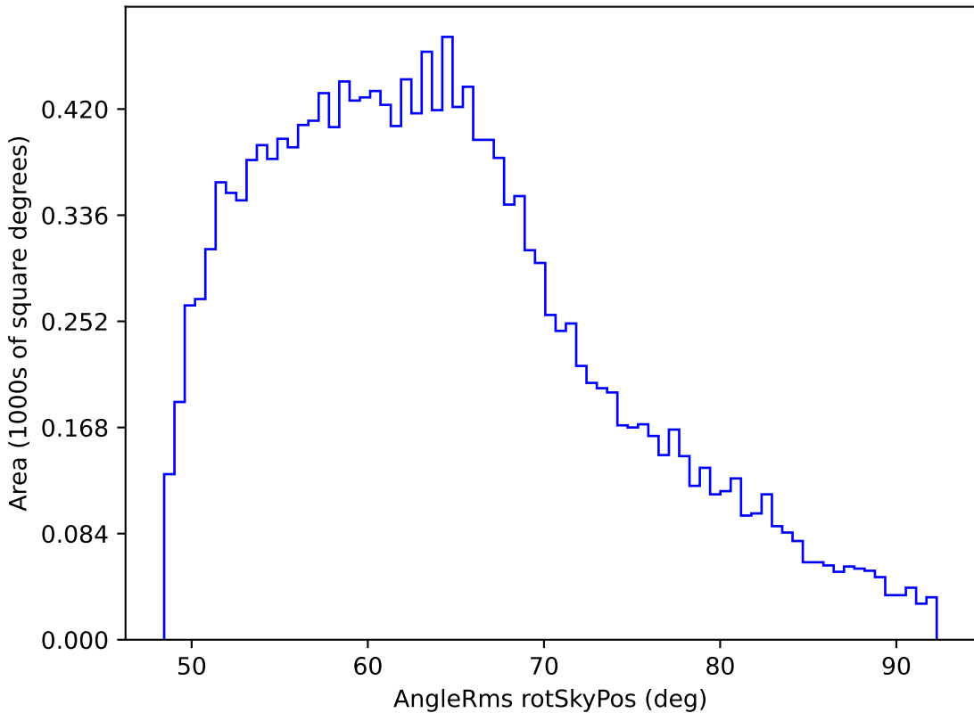
early_u_fpextra2.0_v3.4_10yrs WFD i band: AngleRms rotSkyPos
