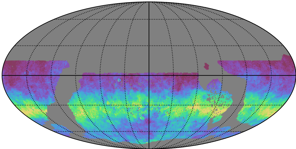
early_u_fpextra2.0_v3.4_10yrs WFD g band: AngleRms rotSkyPos
