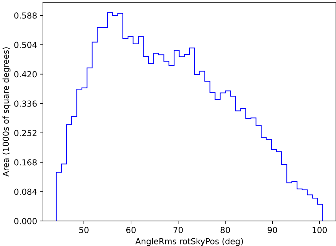
early_u_fpextra2.0_v3.4_10yrs WFD g band: AngleRms rotSkyPos
