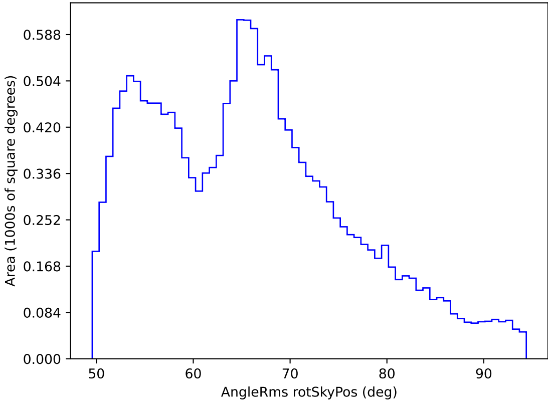
early_u_fpextra2.0_v3.4_10yrs WFD all bands: AngleRms rotSkyPos
