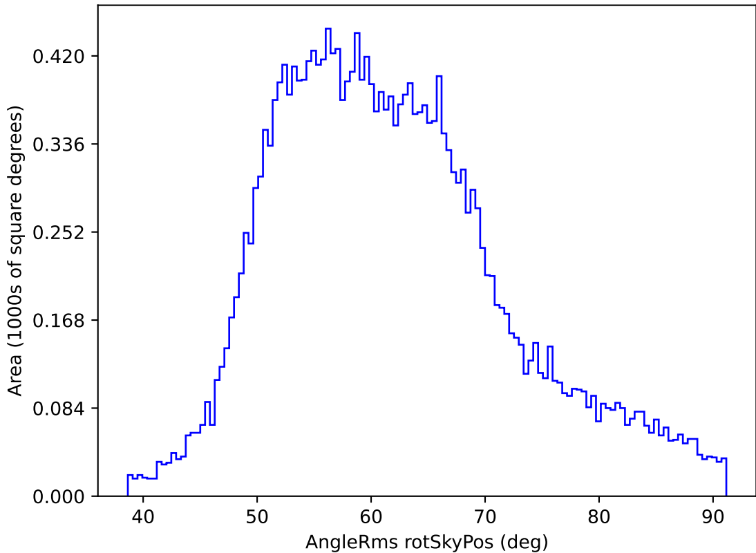
early_u_fpextra2.0_v3.4_10yrs All sky y band: AngleRms rotSkyPos
