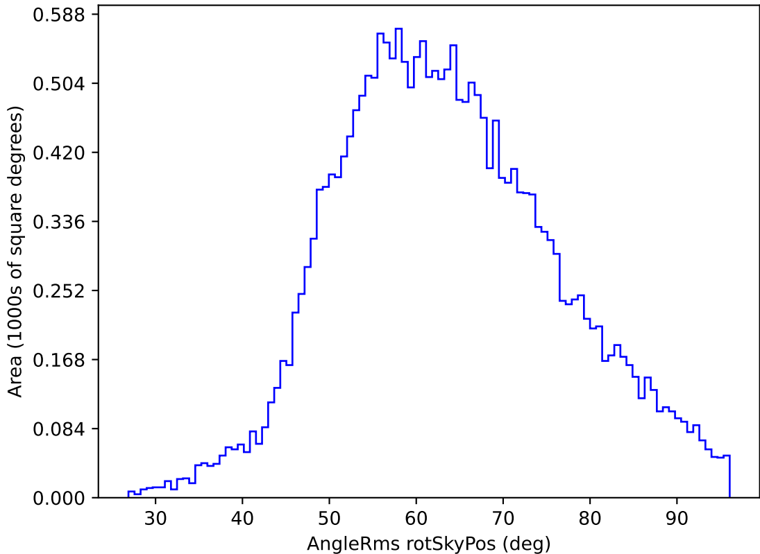
early_u_fpextra2.0_v3.4_10yrs All sky u band: AngleRms rotSkyPos
