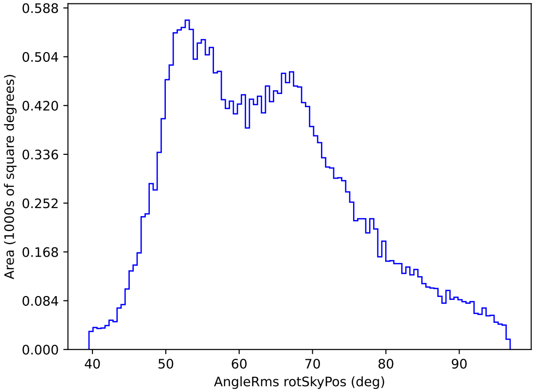
early_u_fpextra2.0_v3.4_10yrs All sky r band: AngleRms rotSkyPos
