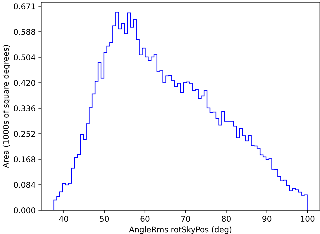
early_u_fpextra2.0_v3.4_10yrs All sky g band: AngleRms rotSkyPos
