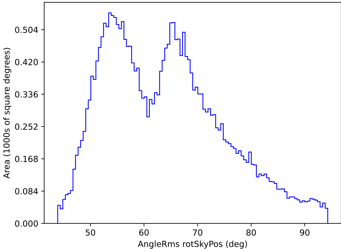
early_u_fpextra2.0_v3.4_10yrs All sky all bands: AngleRms rotSkyPos
