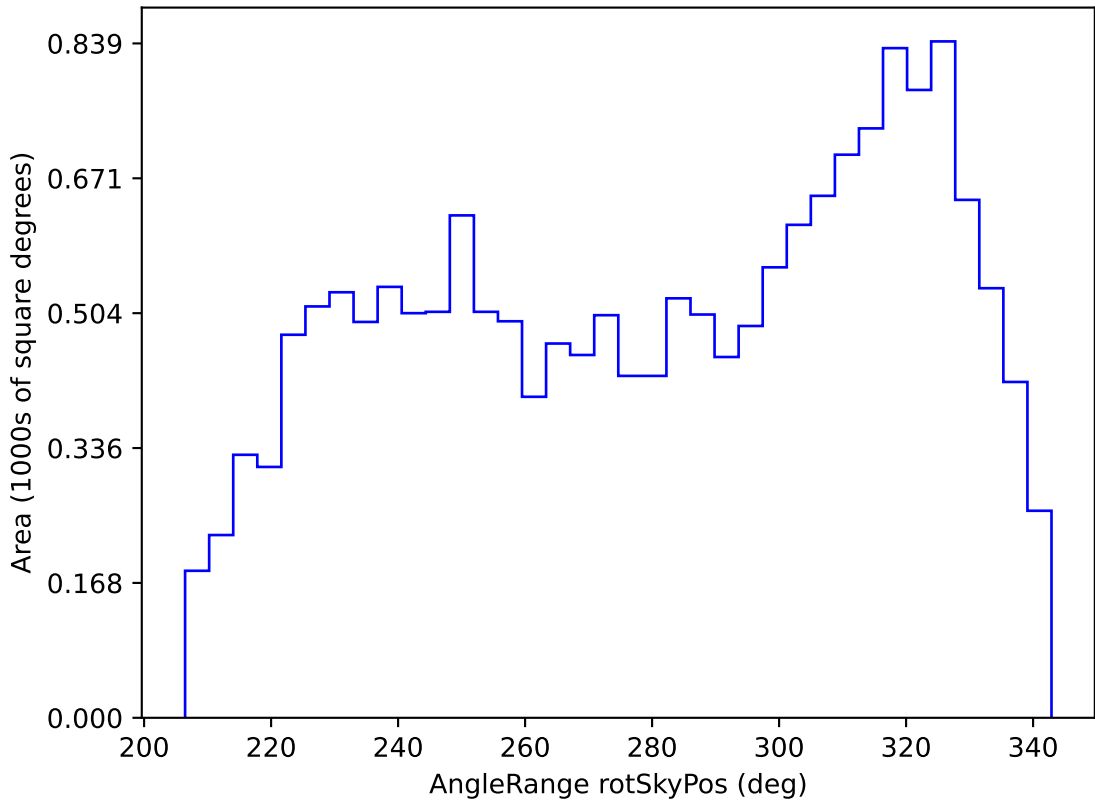
early_u_fpextra2.0_v3.4_10yrs WFD z band: AngleRange rotSkyPos
