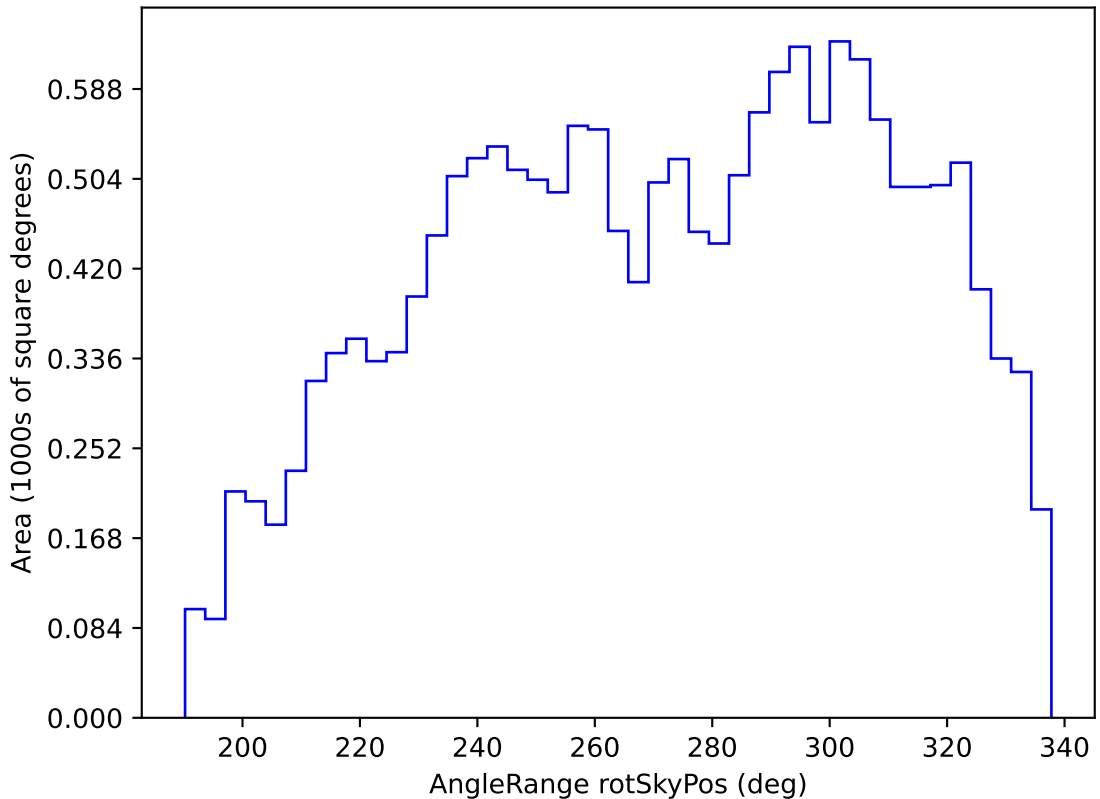
early_u_fpextra2.0_v3.4_10yrs WFD y band: AngleRange rotSkyPos
