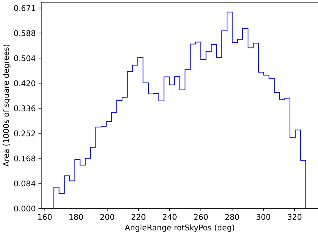
early_u_fpextra2.0_v3.4_10yrs WFD u band: AngleRange rotSkyPos
