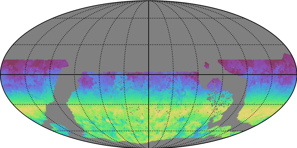
early_u_fpextra2.0_v3.4_10yrs WFD r band: AngleRange rotSkyPos
