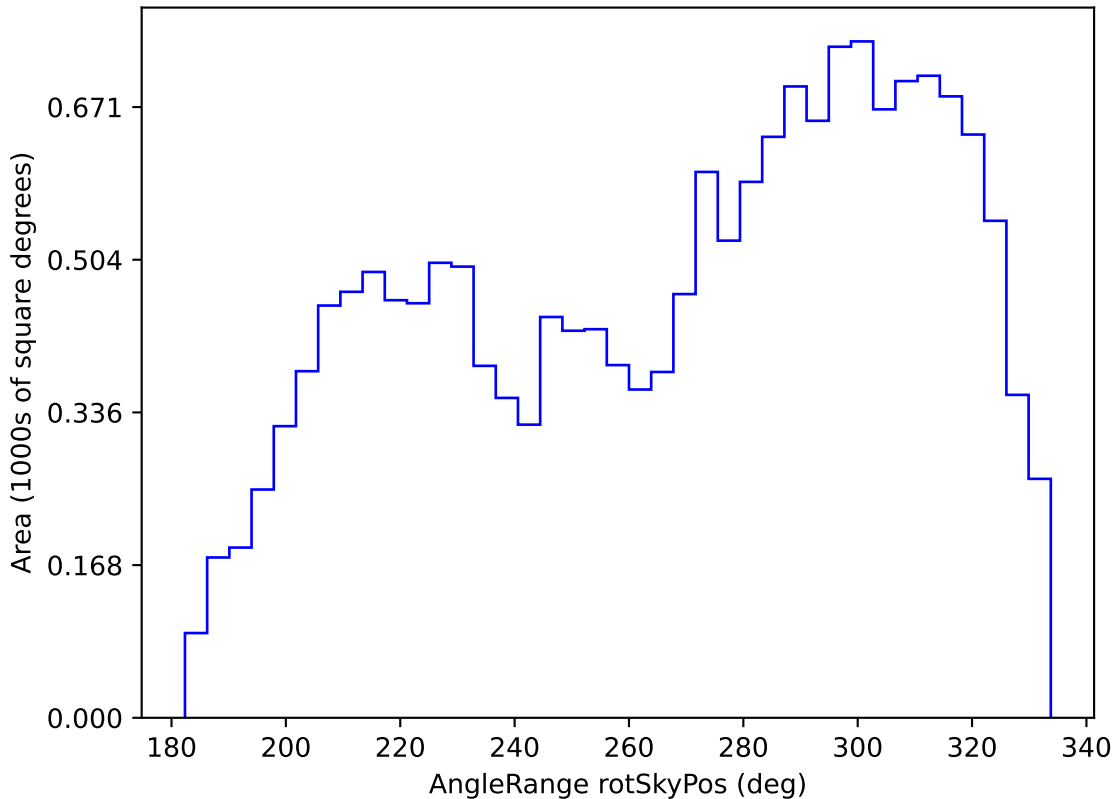
early_u_fpextra2.0_v3.4_10yrs WFD g band: AngleRange rotSkyPos
