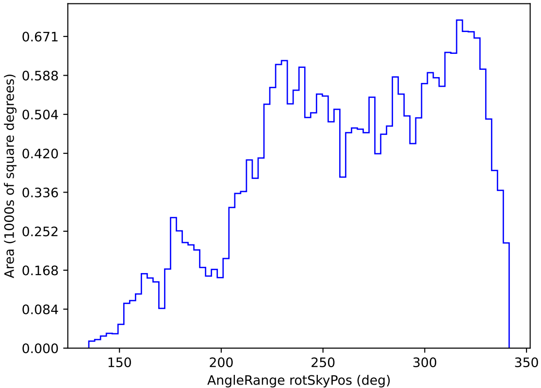
early_u_fpextra2.0_v3.4_10yrs All sky z band: AngleRange rotSkyPos
