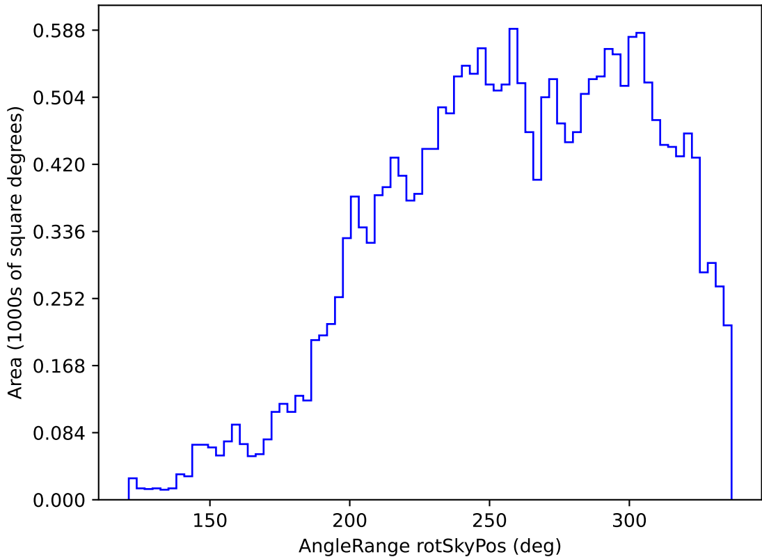
early_u_fpextra2.0_v3.4_10yrs All sky y band: AngleRange rotSkyPos
