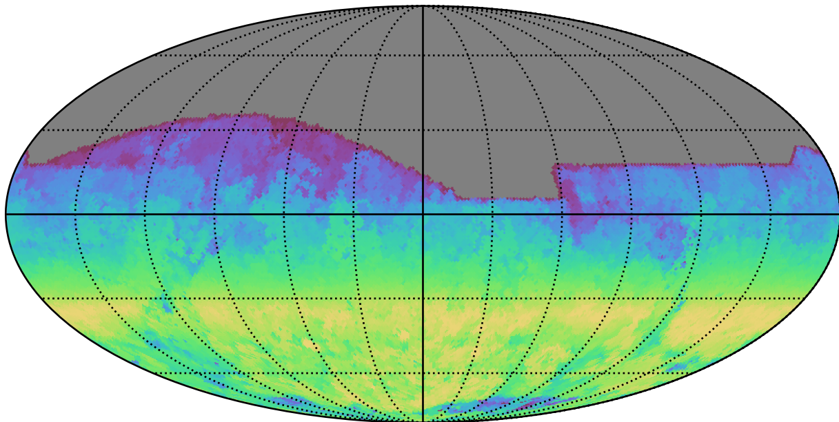
early_u_fpextra2.0_v3.4_10yrs All sky r band: AngleRange rotSkyPos
