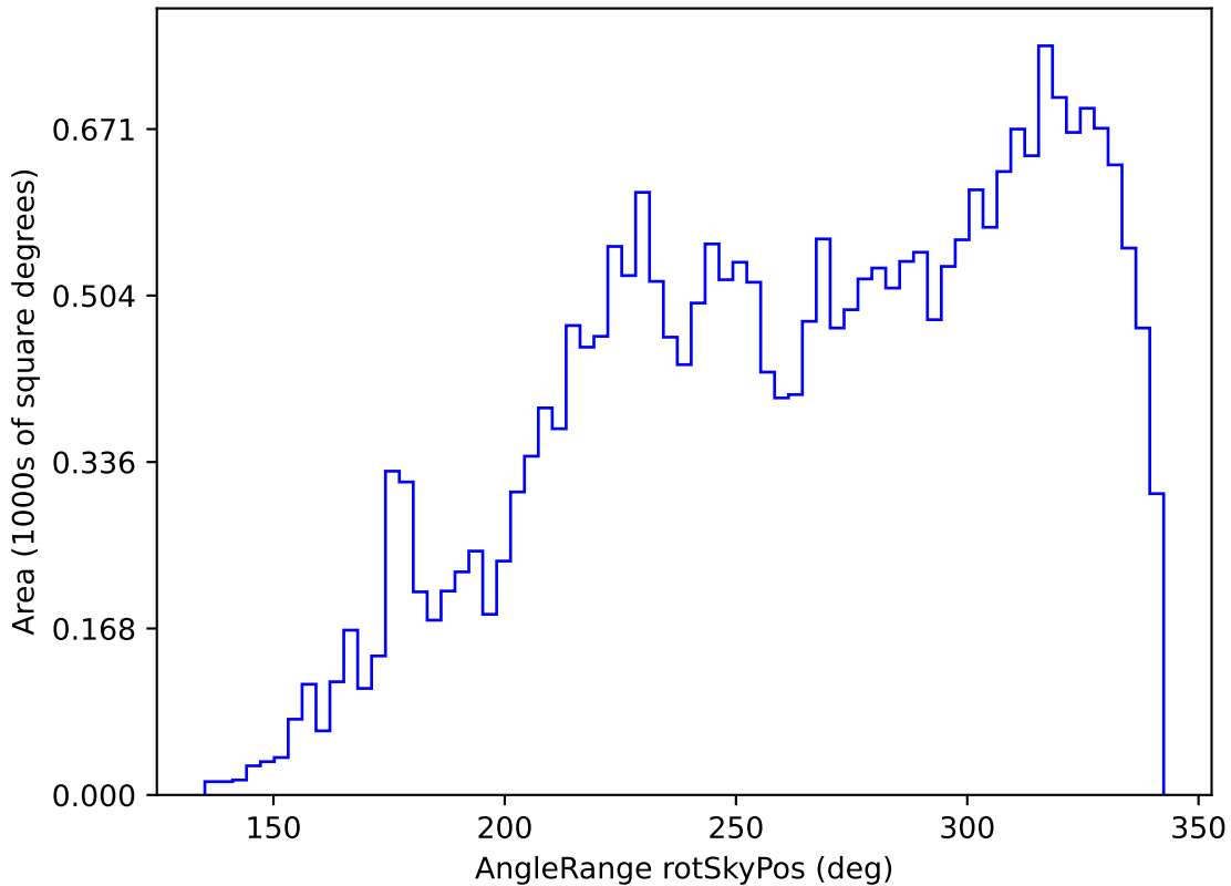
early_u_fpextra2.0_v3.4_10yrs All sky r band: AngleRange rotSkyPos
