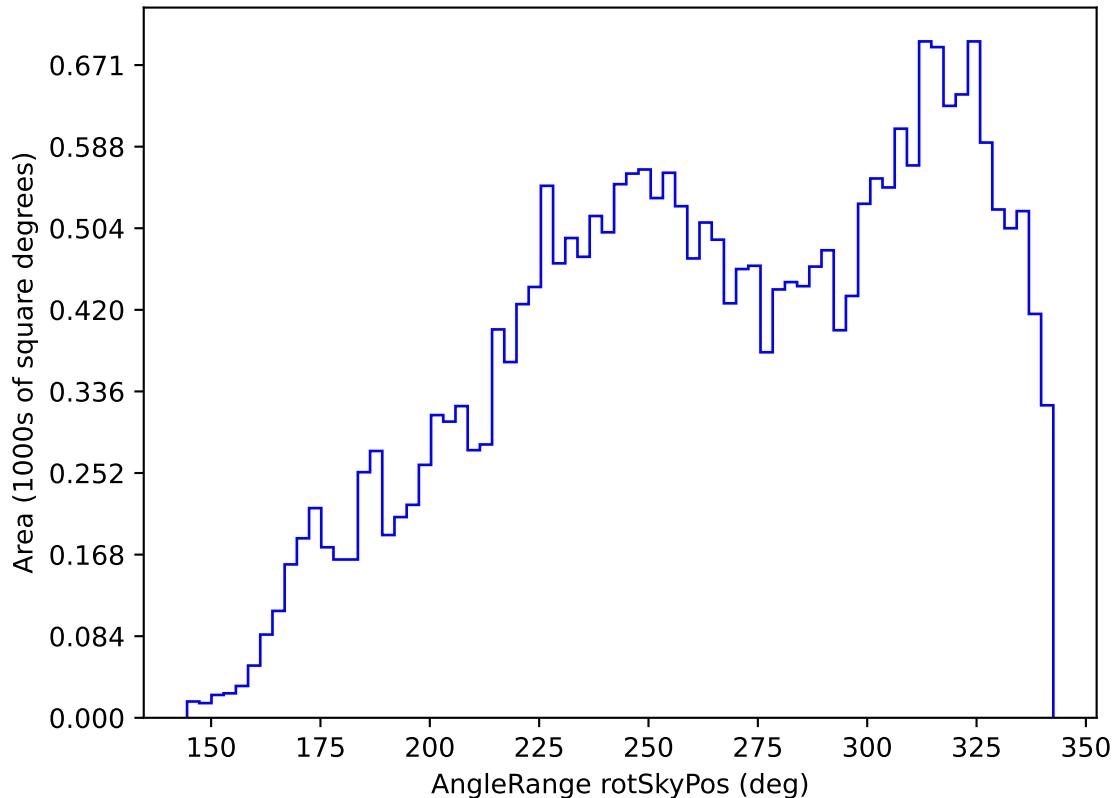
early_u_fpextra2.0_v3.4_10yrs All sky i band: AngleRange rotSkyPos
