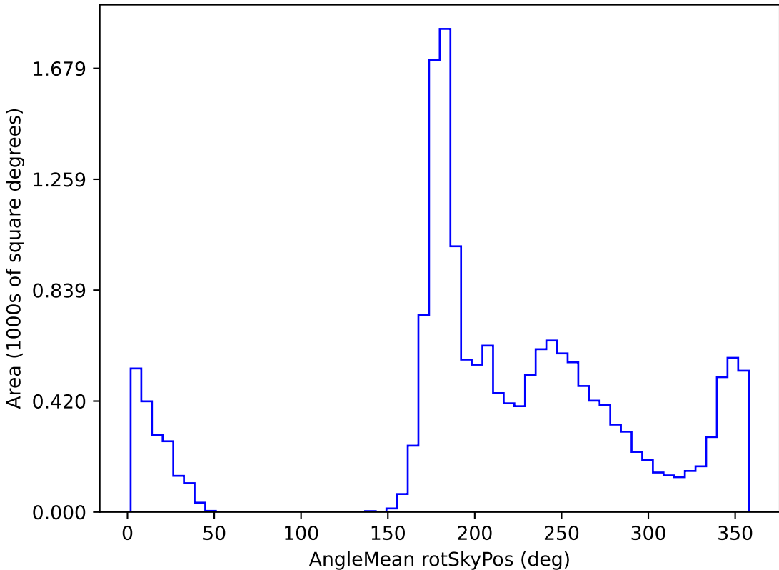
early_u_fpextra2.0_v3.4_10yrs WFD z band: AngleMean rotSkyPos
