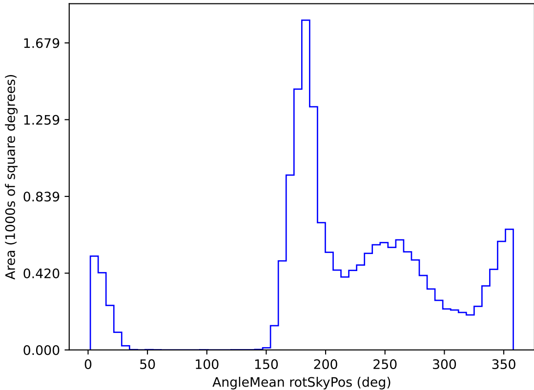
early_u_fpextra2.0_v3.4_10yrs WFD y band: AngleMean rotSkyPos
