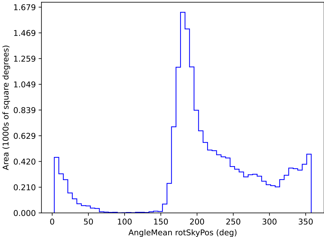
early_u_fpextra2.0_v3.4_10yrs WFD u band: AngleMean rotSkyPos
