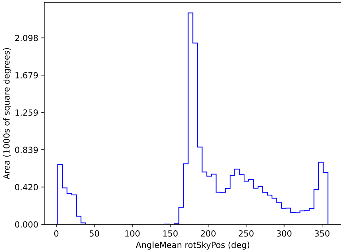
early_u_fpextra2.0_v3.4_10yrs WFD all bands: AngleMean rotSkyPos
