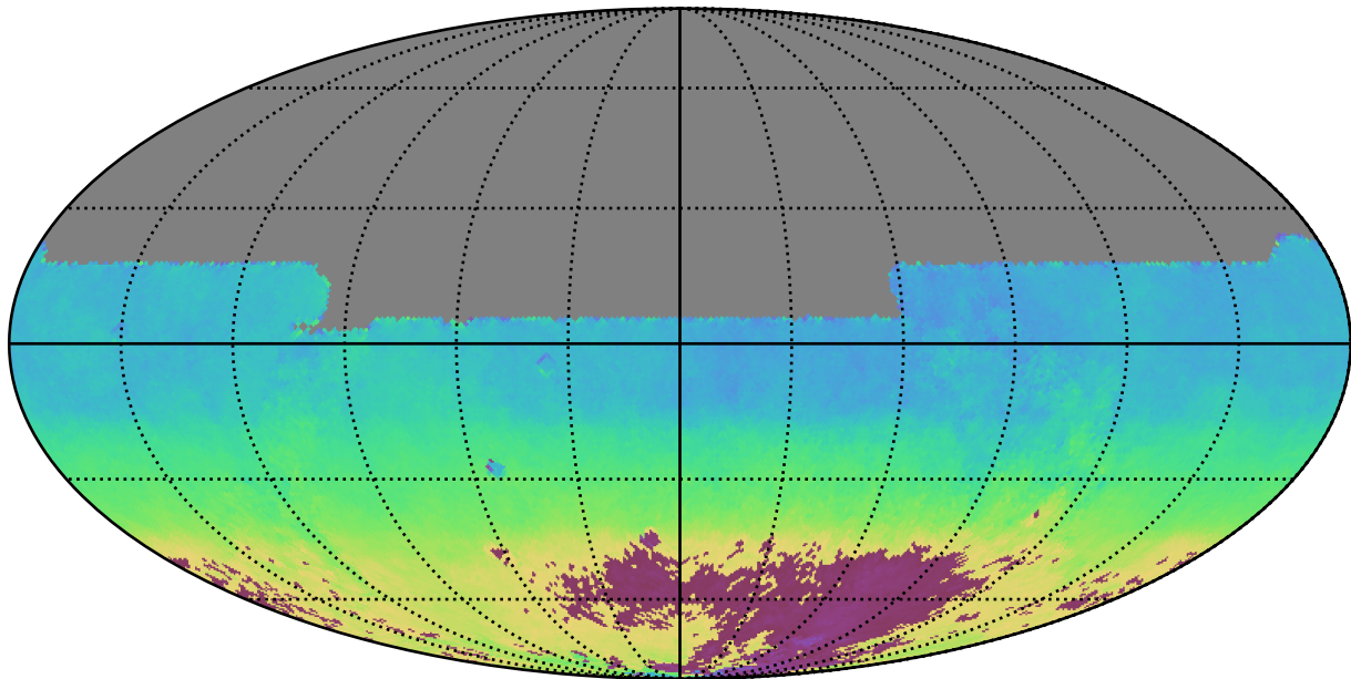
early_u_fpextra2.0_v3.4_10yrs All sky y band: AngleMean rotSkyPos
