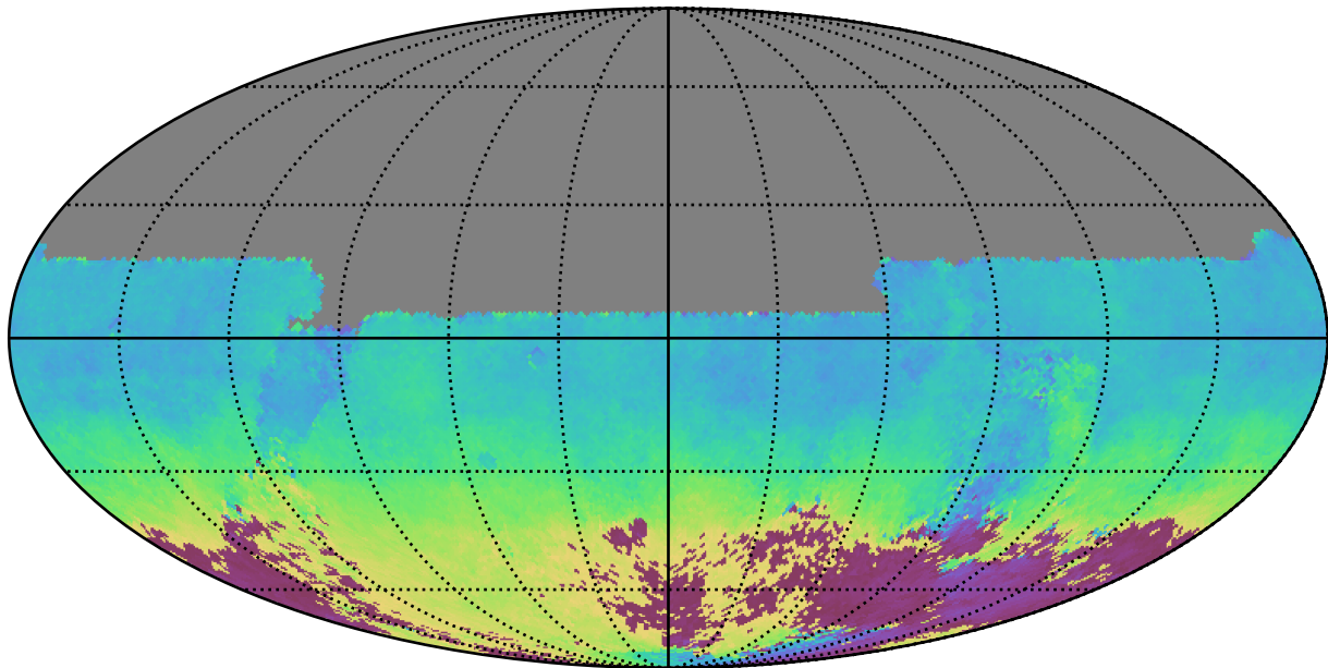
early_u_fpextra2.0_v3.4_10yrs All sky u band: AngleMean rotSkyPos
