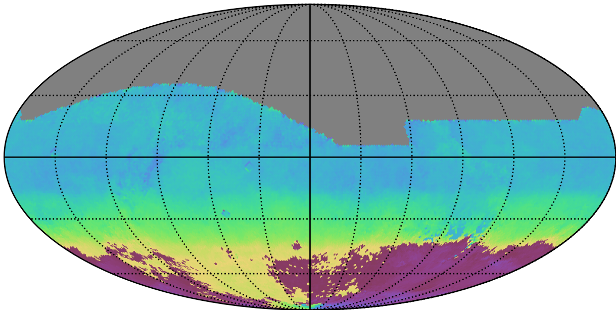
early_u_fpextra2.0_v3.4_10yrs All sky r band: AngleMean rotSkyPos
